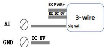
Figure 5 Analog Input
