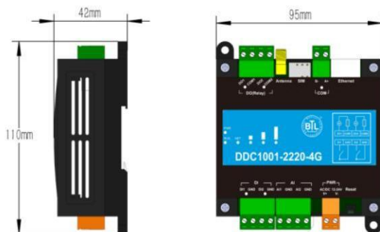
Figure 8 110mm*95mm*42mm(LxWxH) Weight :150g
