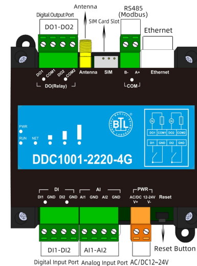
Figure1 Power and Communication Diagram
